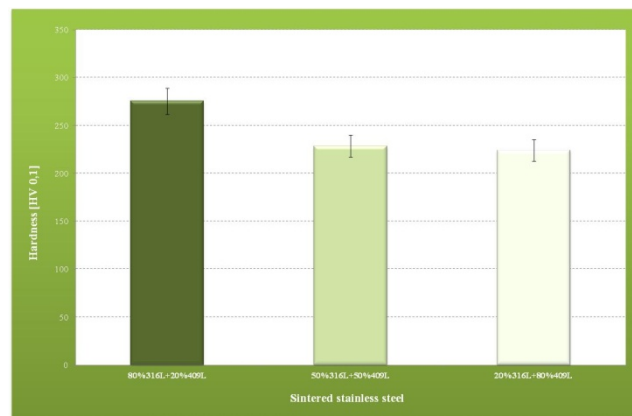
Fig. 3. Microhardness of sintered steel
