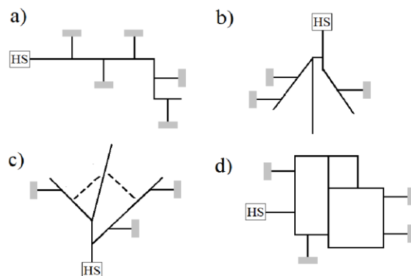
Fig. 2. Basic shape of a horizontal heating networks: a) line, b) branched (radial), c) branched connecting, d) annular
