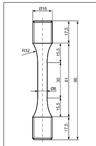
a) specimen for low frequency cyclic loading
