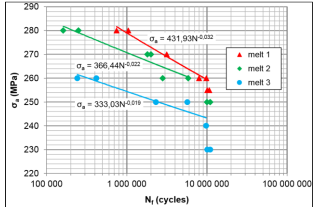
Fig. 4. Wöhler curves \sigma_a = f(N) for low frequency cyclic loading
