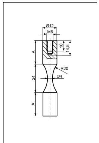
b) specimen for high frequency cyclic loading
