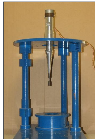
a) ultrasonic fatigue testing equipment KAUP-ZU
